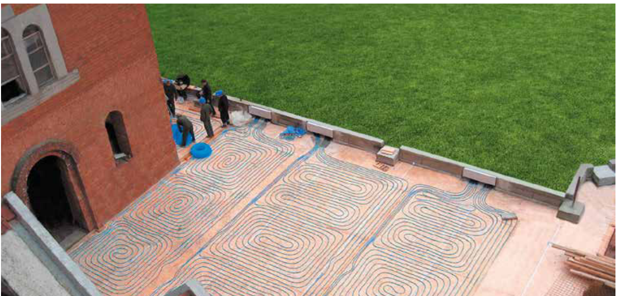
Att. 5. Heating installation of outdoor patio employing KAN-therm system bluePERT pipes.
